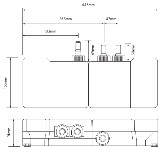
SMARTVALVE
