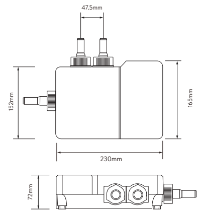
SMARTVALVE
